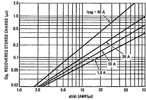
FIGURE 15 - Tj = 150°C
