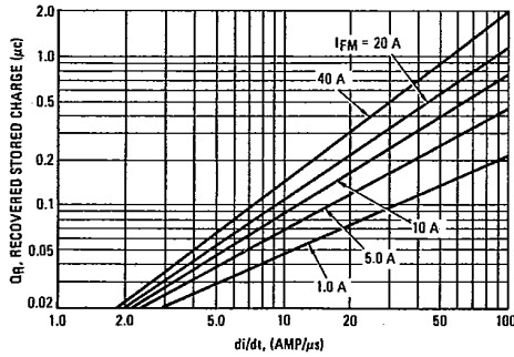
FIGURE 14 - Tj = 100°C
